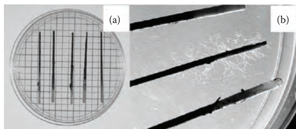
FIGURE 16.10 Toothpick assay. (a) Five toothpicks were removed from soil and placed on a plate of Rhizoctonia selective medium, with 5-mm counting grid underneath. (b) Colony of Rhizoctonia solani growing out of toothpick after 24 h. (From Paulitz, T.C., and Schroeder, K.L., Plant Dis. 89, 767–772, 2005. With permission.)
