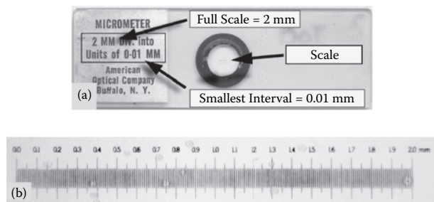
FIGURE 3.11 (a) Stage micrometer and (b) magnified scale of the stage micrometer. The total length of the scale is 2 mm (2000 μm). It is divided into 20 intervals of 0.1 mm or 100 μm (b). Each of these is further divided into intervals of 0.01 mm or 10 μm. (Courtesy of D.T. Webb.)
