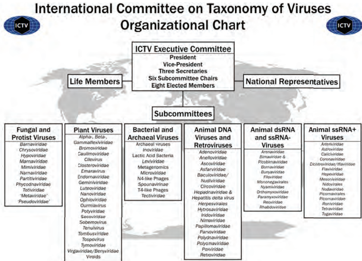
FIGURE 4.5 Organizational chart of the International Committee on Taxonomy of Viruses (ICTV). http://www.ictvonline.org/organization.asp [accessed July 1, 2016].)
