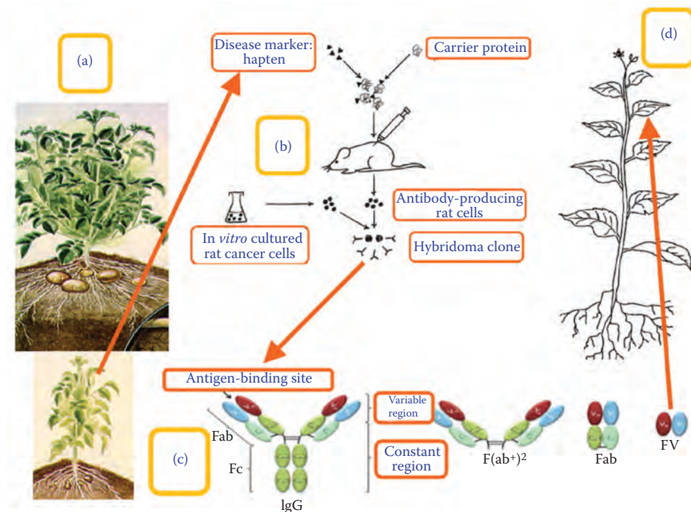
FIGURE 24.6 Immunomodulation. (a) Healthy and pathogen-infected plant. (b) Production of monoclonal antibodies specific for a pathogen protein or hapten. (c) Identification of the nucleotide sequences corresponding to the hypervariable region of the monoclonal antibody. (d) Recombinant production of the selected monoclonal antibody fragment within the plant tissues (plantibody), capable of recognizing and binding to the pathogen protein or hapten. Note: Hybridoma is a hybrid cell resulting from the fusion of a lymphocyte and a tumor cell and used to culture specific monoclonal antibodies.
