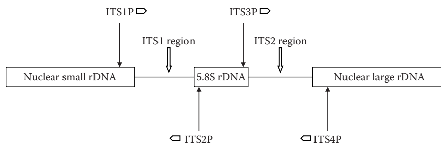
FIGURE 33.4 Diagrammatic representation of internal transcribed spacer (ITS) and ribosomal regions. (Modified from White, T.J.T. et al., Amplification and direct sequencing of fungal ribosomal RNA genes for phylogenetics. In M.A. Innis, D.H. Gelfand, J.J. Sninsky, and T.J. White [eds.], PCR Protocols: A Guide to Methods and Applications , Pages 315–322, San Diego, CA: Academic Press, 1990.) ITS1 and ITS2 are primers for ITS-1 region and ITS3 and ITS4 are primers for ITS-2 region. (From Triganò R. N., M.T. Windham, and A.S. Windham [eds.], Plant Pathology Concepts and Laboratory Exercises , 2nd edition, Boca Raton, FL: CRC Press, 2008.)
