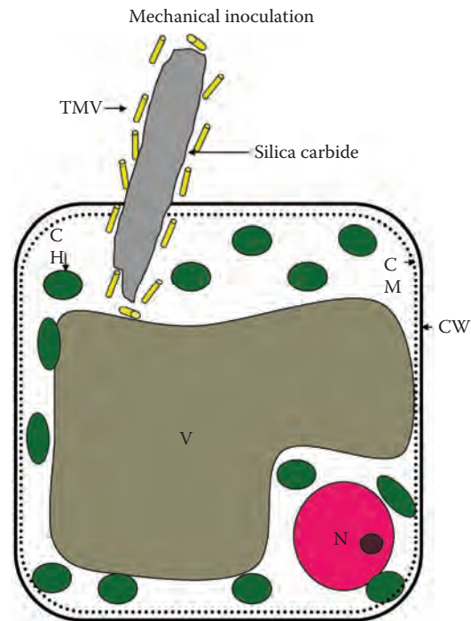
FIGURE 4.17 Mechanical inoculation of plant viruses requires wounding of the plant cell by an abrasive. Silica carbide particles rupture the cell wall (CW) and cell membrane (CM) and allow viruses to enter the cell. Other structures shown in the cell include nucleus (N), chloroplasts (CH), and central vacuole (V). (Courtesy of M. Langham.)
