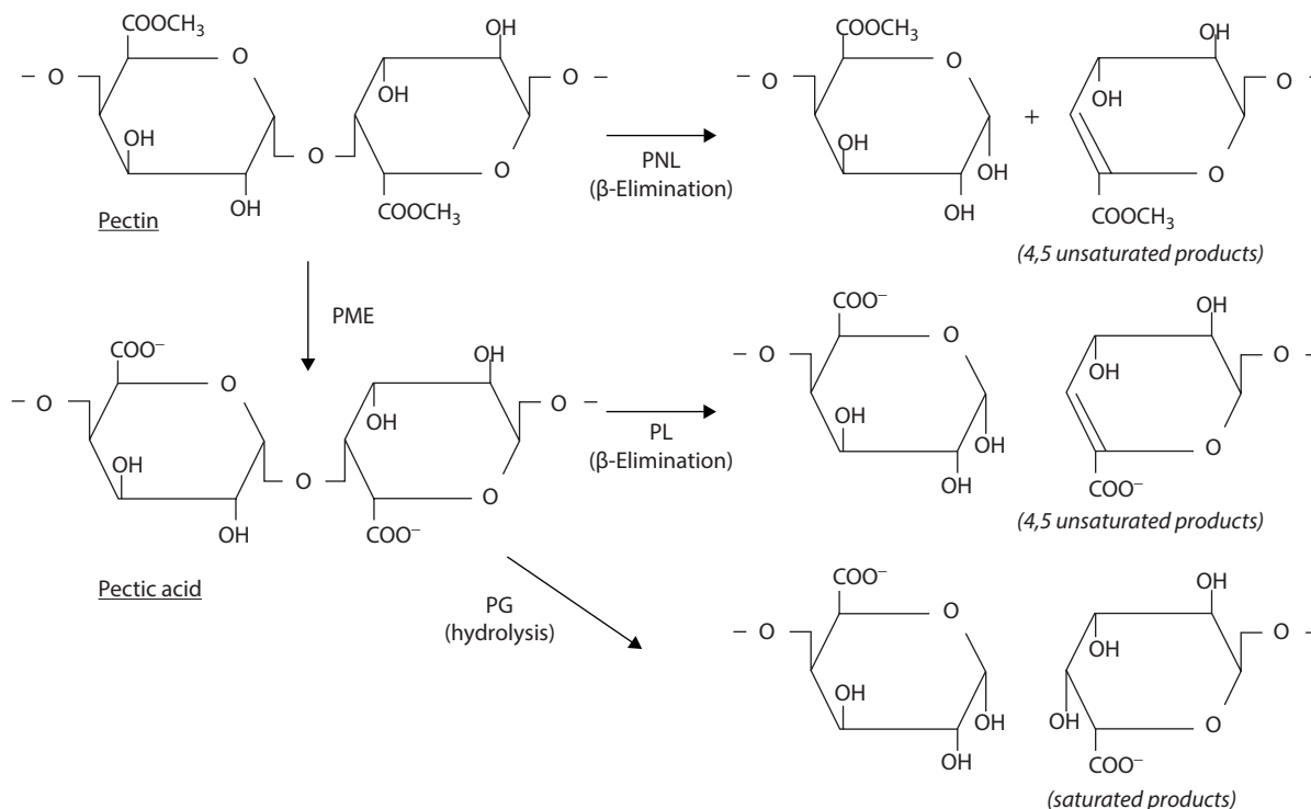
FIGURE 19.1 Cleavage of \alpha -1,4 glycosidic bonds by various pectinases. PG, polygalacturonase; PME, pectin methyltransferase; PL, pectic acid lyase; PNL, pectin lyase.
