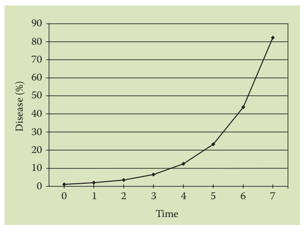
FIGURE 22.5 Exponential model of disease development over time.
