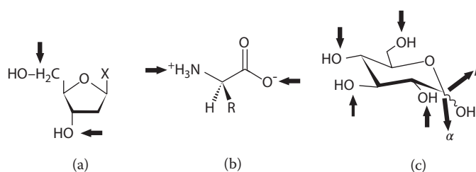
FIGURE 24.8 Illustration of the linkage points (arrows) for oligomer formation in biomolecules. In comparison with the phosphodiester and peptide bonds, strictly constrained in their capacity for oligomer formation, a large panel of glycosidic linkages can be formed. The phosphodiester bond in nucleic acid biosynthesis (a) and the peptide bond in protein biosynthesis (b) yield linear oligomers. In contrast, the glycosidic linkage in oligosaccharides (c) can involve any hydroxyl group on the second monomer, opening the way to both linear and branched structures. This unique property is symbolized by arrows directed toward the hydroxyl groups. The anomeric configuration ( \alpha or \beta ) in chain elongation can vary, as symbolized by two bold arrows pointing away from the molecule. (Extracted from Ferreira, R. et al., Eur. J. Plant Pathol. , 133, 117–140, 2012; Originally from Gabius H.-J., The Sugar Code: Fundamentals of Glycosciences , Wiley-VCH Verlag GmbH & Co. KGaA, Weinheim, 2009.)
