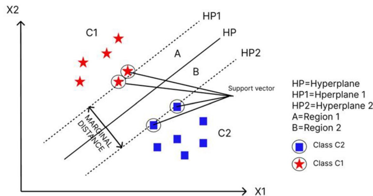
Figure 8. SVM illustration.
