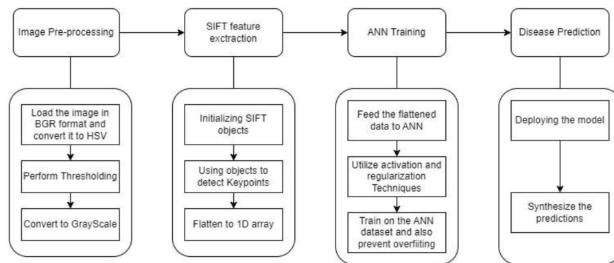
Figure 13. ANN + SIFT.
