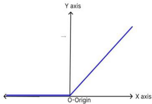
Figure 9. ReLu function.
