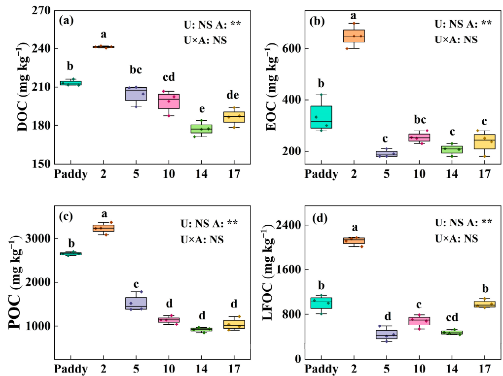
Figure 1. Effects of different land uses on the content of organic C fractions. The 2, 5, 10, 14, and 17 represent the cultivation durations of the areca nut plantations. DOC: dissolved organic carbon, EOC: easily oxidizable organic carbon, POC: particulate organic carbon, LFOC: light fraction organic carbon, and MBC: soil microbial carbon. Different lowercase letters in the figure represent significant differences between treatments ( p < 0.05 ). In the results of two-factor ANOVA, U represents different utilization methods and A represents time treatment. U \times A represents the interaction effect of different utilization modes and time processing; NS: no significant difference; **: p < 0.01 . (a–d) indicates the subgraph number in the caption.
