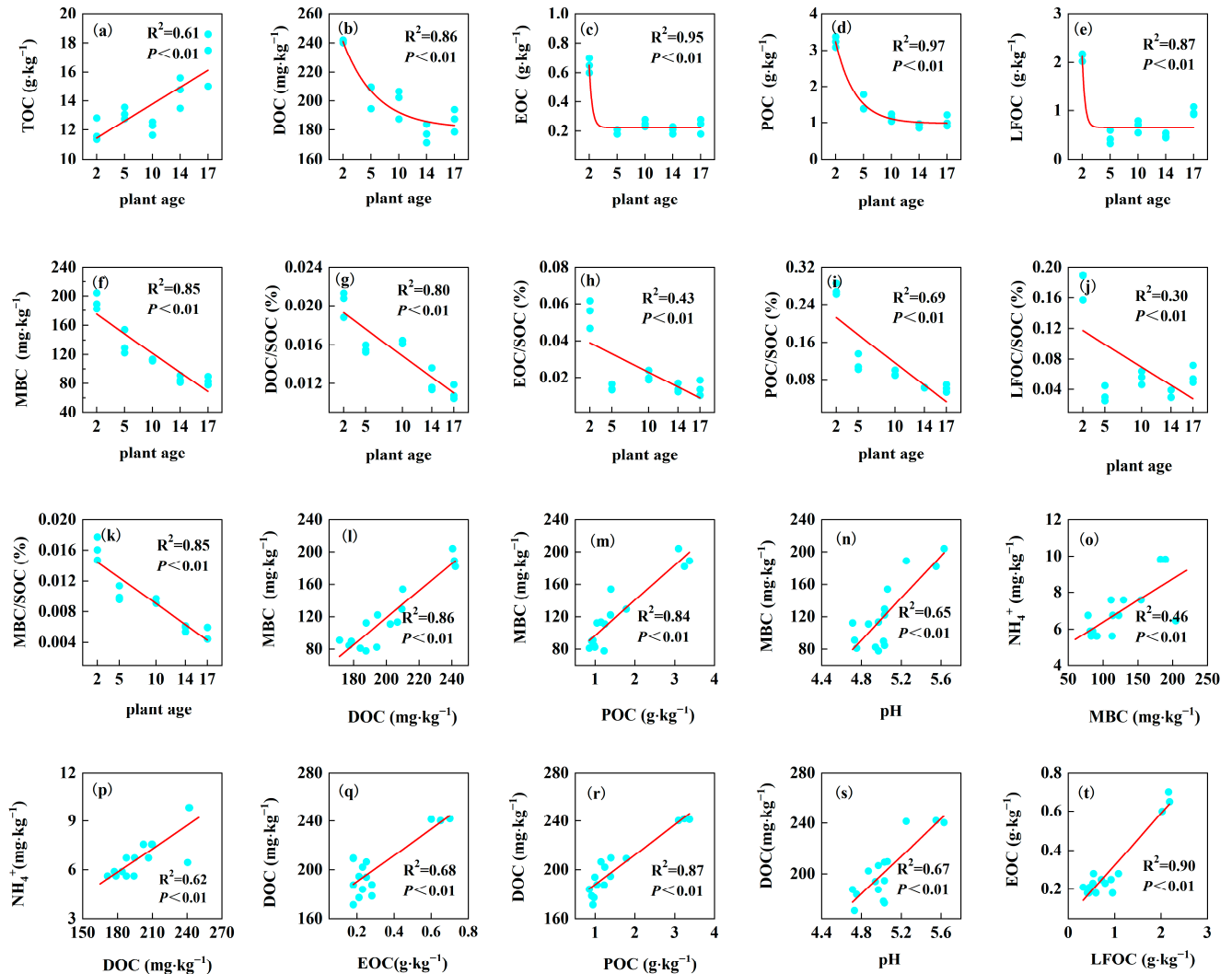
Figure 2. Correlation between planting years of areca nut and organic C and its fractions. Plant age represents the cultivation durations of the areca nut plantations. TOC: soil organic carbon, \text{NH}_4^+ : soil ammonium-nitrogen, DOC: dissolved organic carbon, EOC: easily oxidizable organic carbon, POC: particulate organic carbon, LFOC: light fraction organic carbon, and MBC: soil microbial carbon. (a–t) indicates the subgraph number in the caption.
