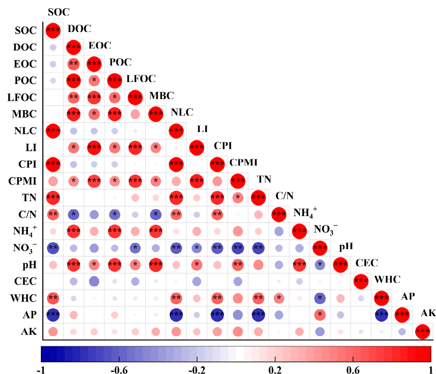
Figure 3. Correlation analysis of soil organic C and its fractions to soil properties. * Significant correlation at 0.05; ** Significant correlation at 0.01; *** Significant correlation at 0.001. SOC: soil organic carbon, DOC: dissolved organic carbon, EOC: easily oxidizable organic carbon, POC: particulate organic carbon, LFOC: light fraction organic carbon, MBC: soil microbial carbon, NLC: nonlabile carbon, LI: carbon pool activity index, CPI: carbon pool index, CPMI: carbon pool management index, TN: soil total nitrogen, C/N: carbon to nitrogen ratio, NH 4 + : soil ammonium–nitrogen, NO 3 − : soil nitrate–nitrogen, CEC: soil cation exchange capacity, WHC: water-holding capacity, AP: soil available phosphorus, AK: soil available potassium.
