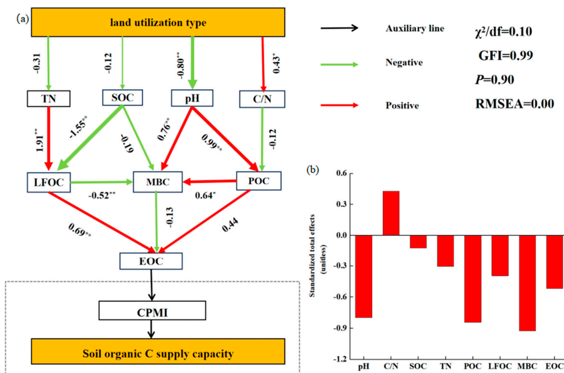
Figure 4. Direct and indirect effects of soil properties and soil C fractions on soil C pool under land-use change. TN: soil total nitrogen, SOC: soil organic carbon, C/N: carbon to nitrogen ratio, POC: particulate organic carbon, LFOC: light fraction organic carbon, MBC: soil microbial carbon, and EOC: easily oxidizable organic carbon. Line width indicates normalized path coefficient strength. Black arrows and red arrows indicate positive and negative significant relationships. \chi^2/df , chi-square/degrees of freedom; p, probability level; GFI, goodness-of-fit index; RMSEA, root mean squared error of approximation. Significance levels of each predictor are p < 0.01 . * Significant correlation at 0.05; ** Significant correlation at 0.01; (a,b) indicates the subgraph number in the caption.
