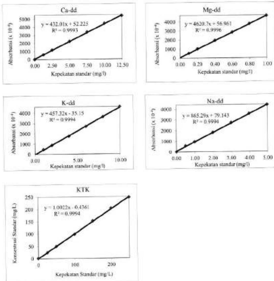
Gambar 36. Linearitas
