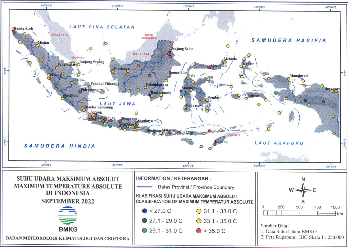
Gambar 1.2 Monitoring Suhu Udara Maksimum Absolut September 2022
