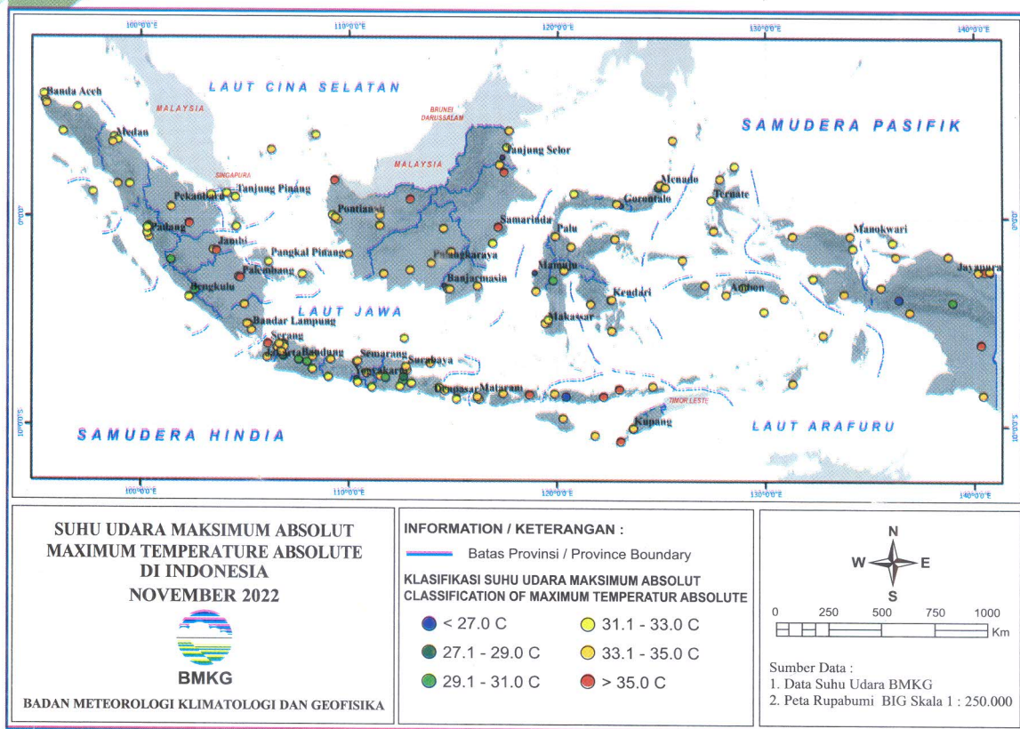
Gambar 1.4 Monitoring Suhu Udara Maksimum Absolut November 2022
