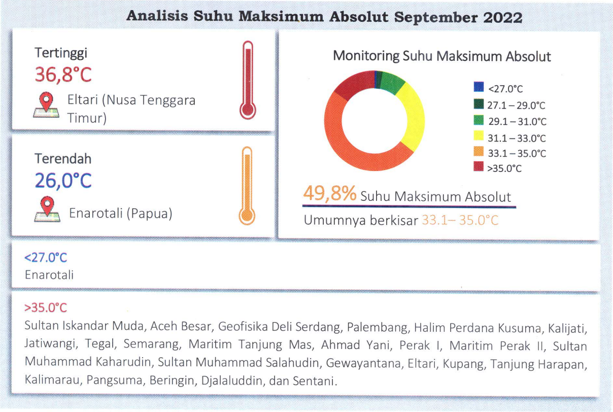
Gambar 1.2 Monitoring Suhu Udara Maksimum Absolut September 2022
